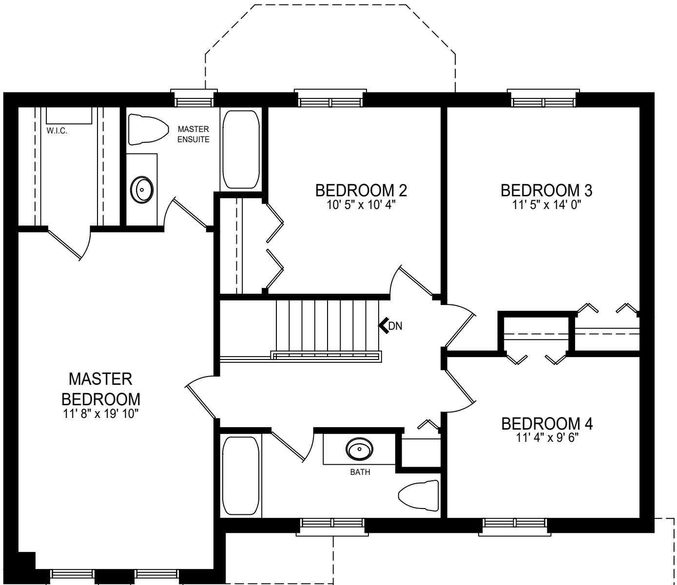
SECOND FLOOR PLAN APPROX. 1,035 SQ.FT.
